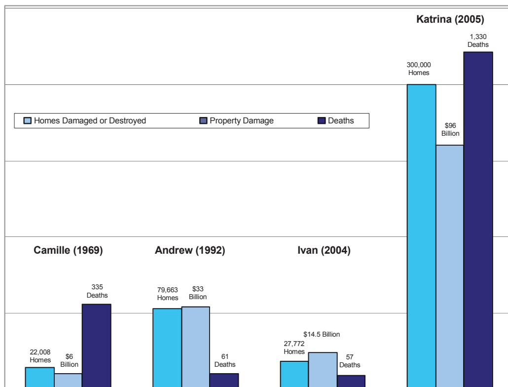
Figure 1.2: Hurricane Katrina Compared to Hurricanes Ivan, Andrew, and Camille 27
